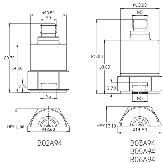
Fig_3 Dimensions of BXXA94
