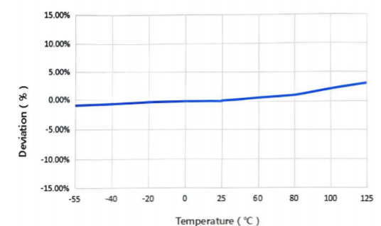
Fig_2 Typical Temperature Response
